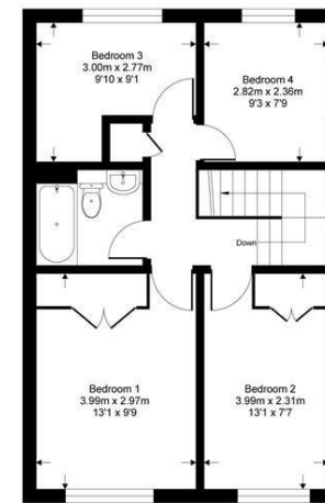
First Floor = 47.1 sqm / 508 sqft
